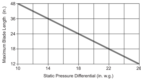
Damper Design Limitations
